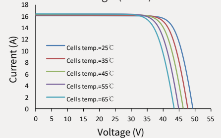
Current-Voltage (635W)
